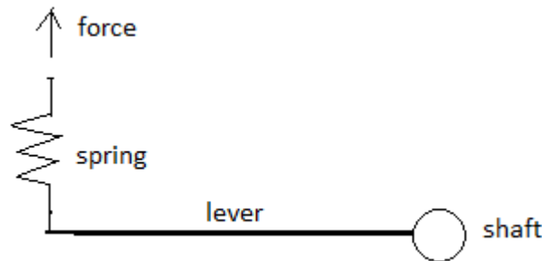
Figure 3. Free Body Diagram of the measurement of Torque
