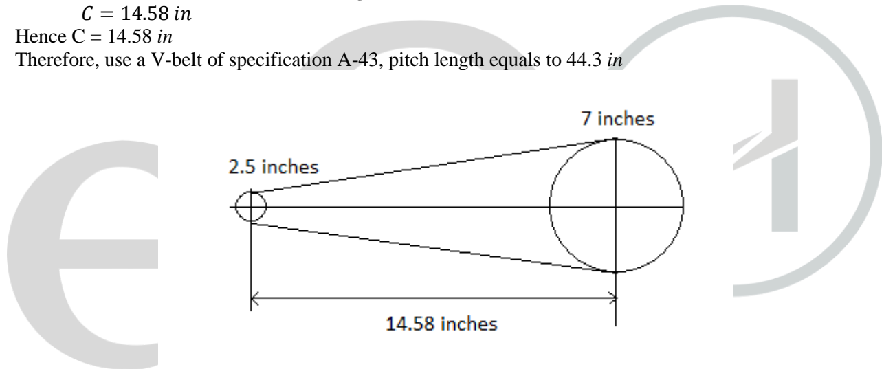
Figure 5. Free Body Diagram of Motor Pulley and the Pulley Connected to the Shaft of Steel Roller
